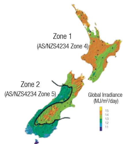
AS/NZS4234 Climate Zones (Solar)
