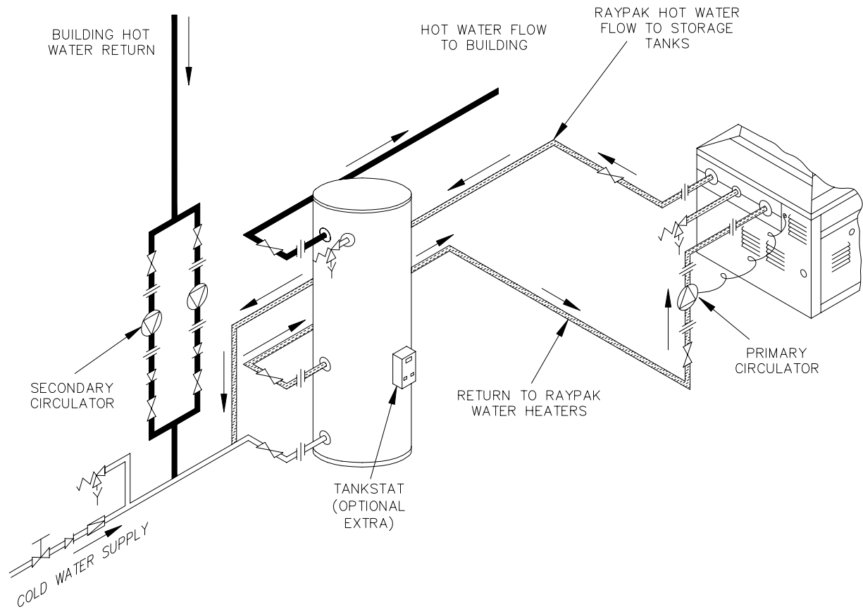
RAYPAK - SINGLE WATER HEATER, SINGLE TANK
