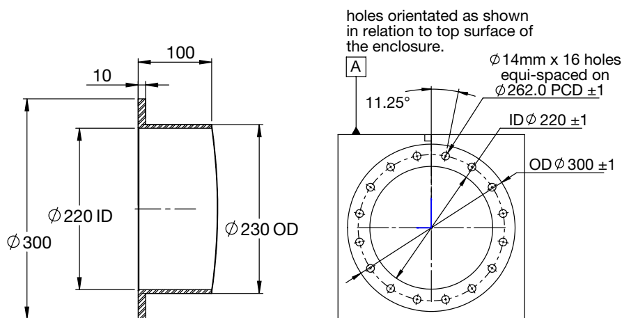
RT Series tank and Heating Unit flange details
