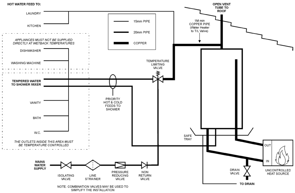
DIAGRAM 3 - Typical 'Wetback' Installation
