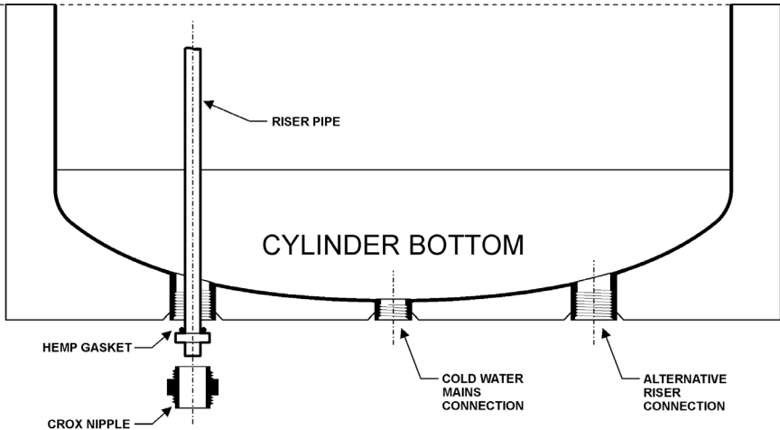
DIAGRAM 4 - 'Wetback' bottom entry cylinder 'Riser' installation
