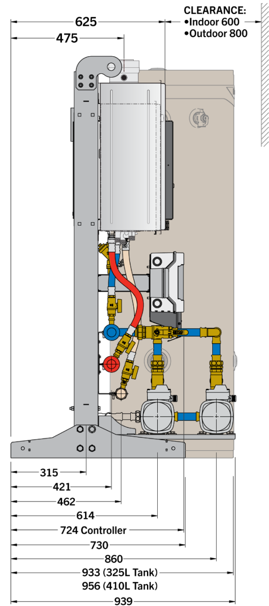
Tankpak Series 4 Drawing (Floor Mount Side View)
