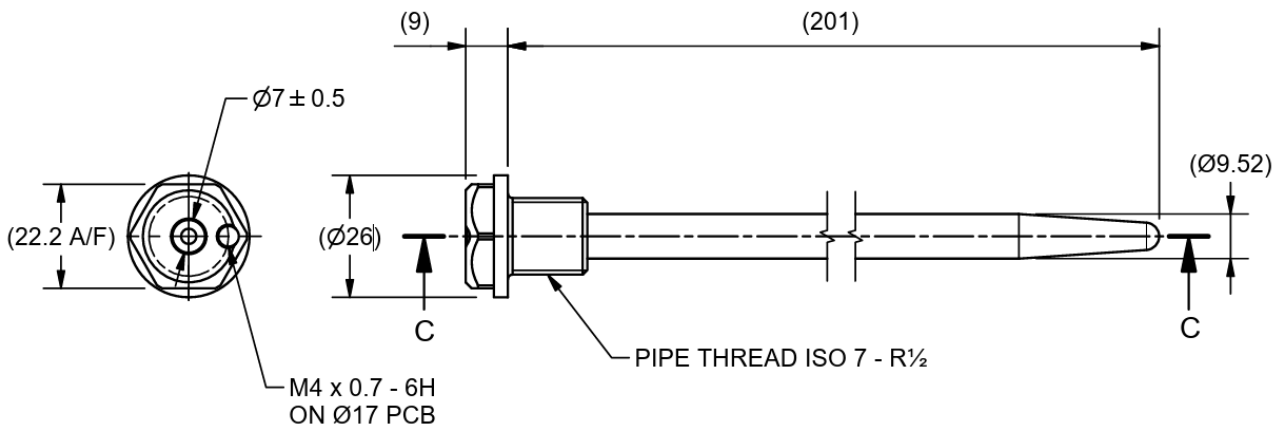
Thermowell Dimensions
