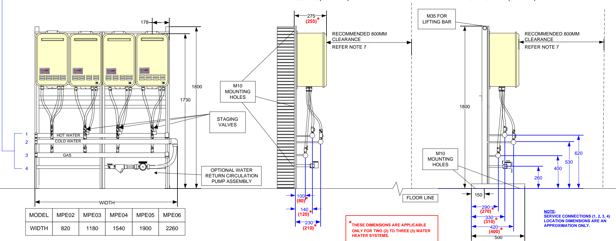
SIDE VIEW WALL MOUNTING (STANDARD)
