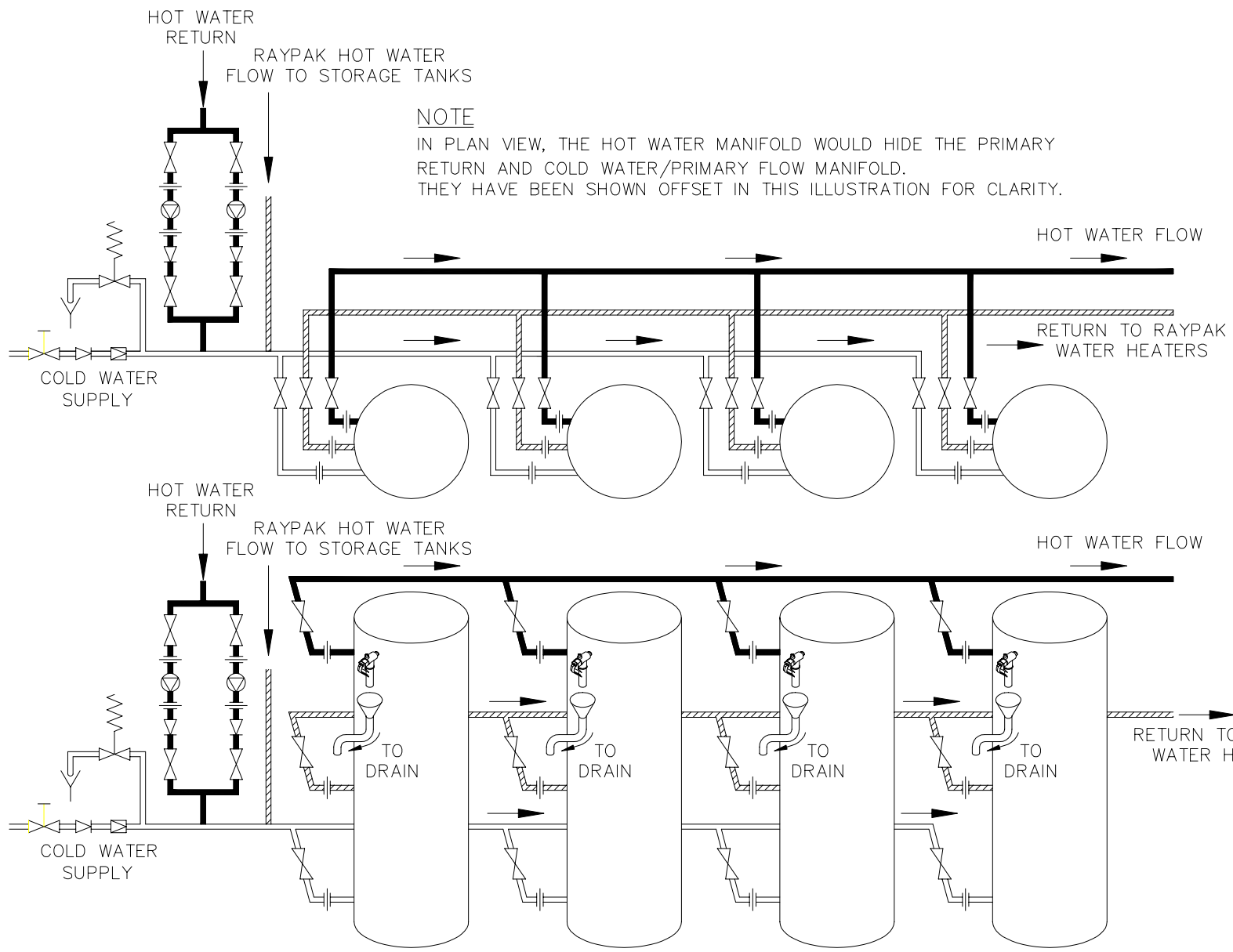
RHEEM 610 SERIES STORAGE TANKS WITH RAYPAK WATER HEATER TYPICAL INSTALLATION
