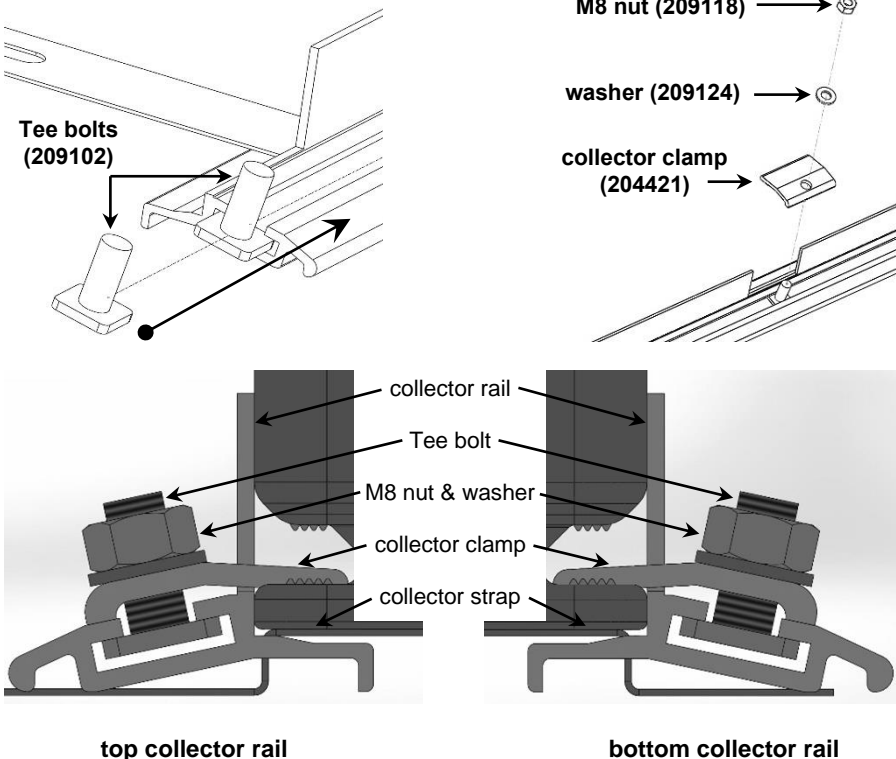
DETAIL D – CLAMPING COLLECTOR TO COLLECTOR RAIL
